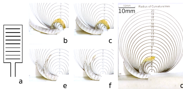
Figure 4. High frequency actuation: (a) Digital design of the tested sample. (b-f) The oscillation amplitude of tested sample when actuated at 1 Hz, 5 Hz, 10 Hz, 20 Hz, and 30 Hz. The air pressure is 2 bar and one side is covered with tape for better reversibility.
