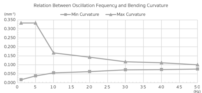
Figure 5. Relation between oscillation frequency and bending curvature
