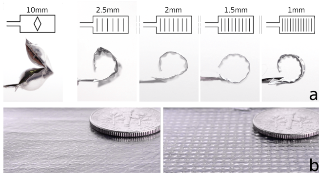
Figure 3. High resolution shape change: (a) Shape change is getting smoother as chambers becomes narrower. (b) Millimeter scale texture change, the size of each dots is ~1 mm × 1 mm.
